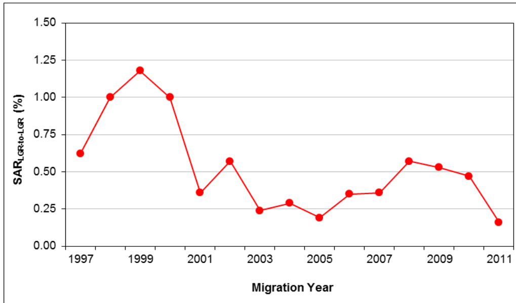
Figure 9. Weighted SAR LGR-10-LGR for Dworshak NFH spring Chinook (1997–2011). Migration year 2011 is incomplete for yearling Chinook, with Age 2-salt adult returns through 9/15/2013.
