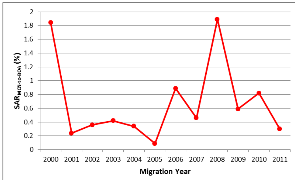
Figure 3. Overall SAR MCN-to-BOA (without jacks) for Leavenworth NFH spring Chinook (2000–2011). Migration year 2011 is incomplete for yearling Chinook, with Age 2-salt adult returns through 9/15/2013.
