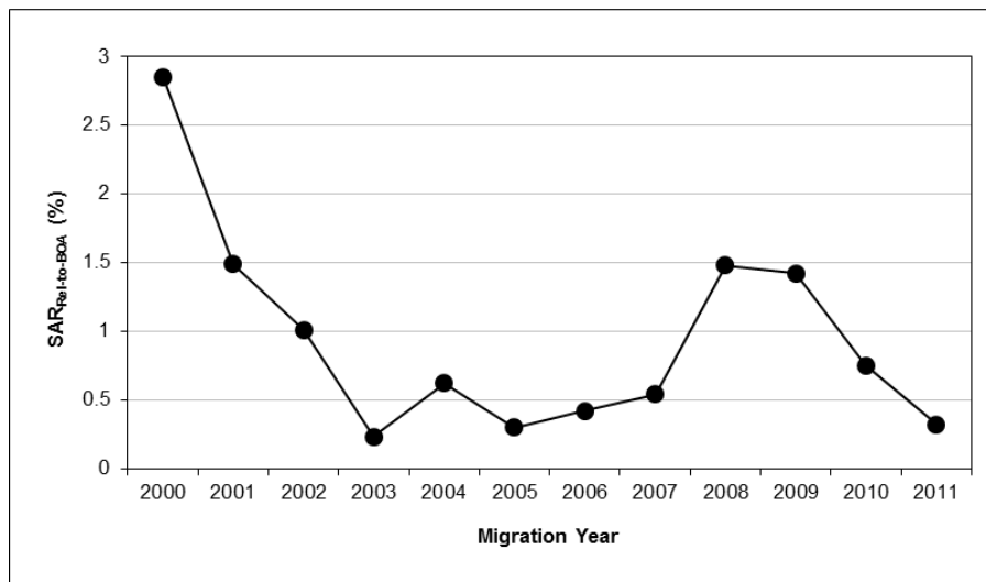
Figure 2. Overall SAR Rel-to-BOA for Carson NFH spring Chinook (2000–2011). Migration year 2011 is incomplete for yearling Chinook, with Age 2-salt adult returns through 9/15/2013.
