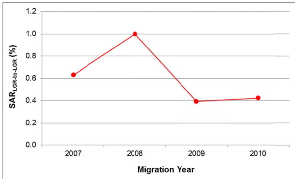
Figure 5. Weighted SAR LGR-10-LGR for Sawtooth Hatchery spring Chinook (2007-2010). All release sites are included in the estimates. Adult returns for migration year 2010 are incomplete, with Age 2-salt adult returns through 9/10/2012.
