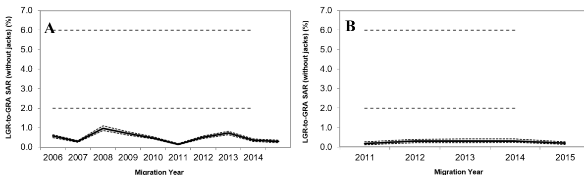
Figure 5. Overall SAR LGR-to-GRA (without jacks) for Clearwater Hatchery spring (A) and summer (B) Chinook (with 90% confidence intervals). The NPCC 2-6% SAR objectives for listed wild populations are shown for reference. Migration year 2015 is incomplete with Age 2-salt adult returns through 9/15/2017.
