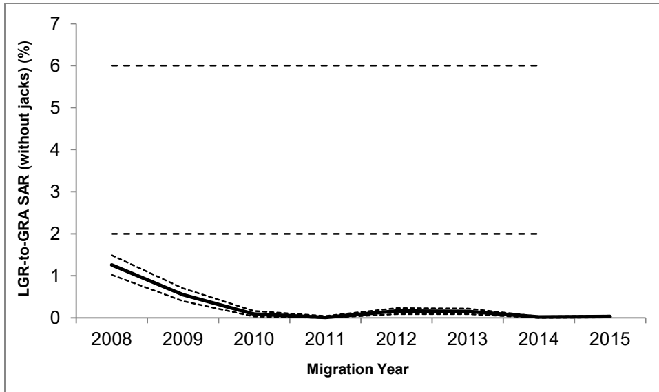
Figure 4. Overall SAR for Pahsimeroi Hatchery summer Chinook (without jacks) (2008–2015) (with 90% confidence intervals). The NPCC 2-6% SAR objectives for listed wild populations are shown for reference. Migration year 2015 is incomplete with Age 2-salt adult returns through 7/22/2017
