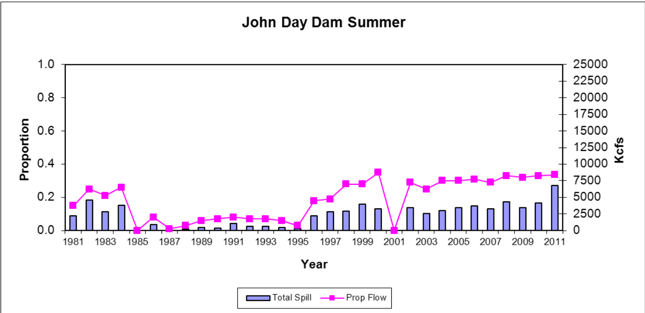
Figure 6. Total spill (Kcfs) for spring (April 10 to June 30) and summer (July 1 - August 31) at John Day Dam, and spill as a proportion of total flow for the same time period.
