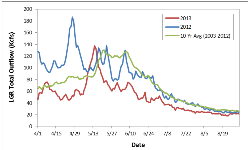
Figure L-1. Average daily flows at Lower Granite Dam 2013, 2012, and the 10-year average
