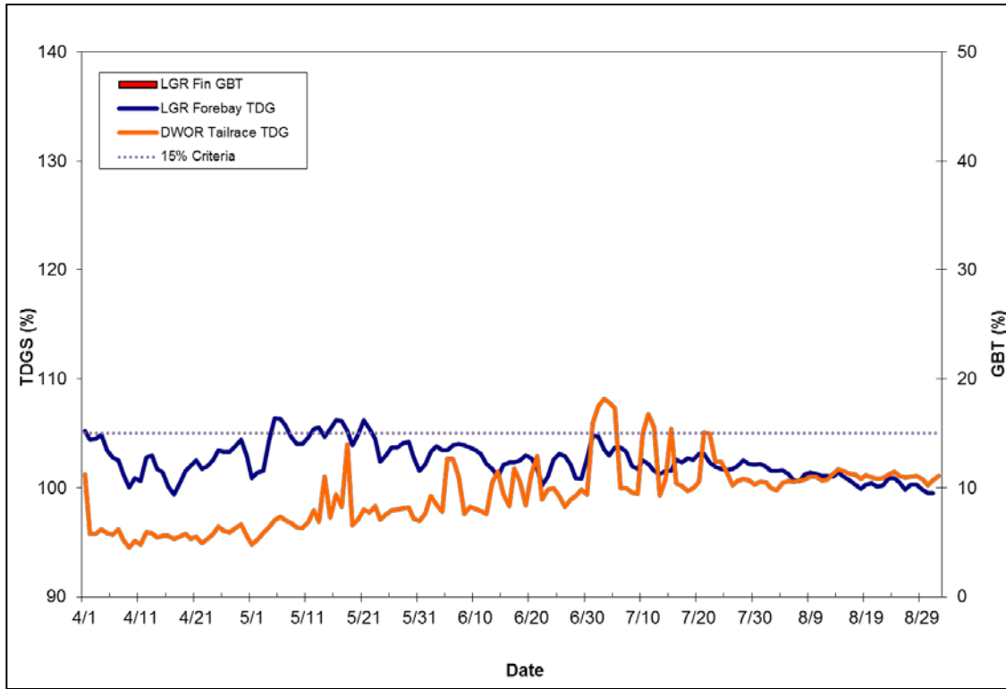
Figure L-3 Percent GBT observed in the sample at Lower Granite Dam
